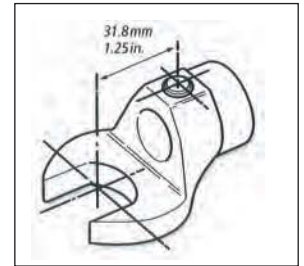
Where the distance between centres differs from 1.25 in (31.8mm) the torque applied will not be as set on the wrench (see page 10)
